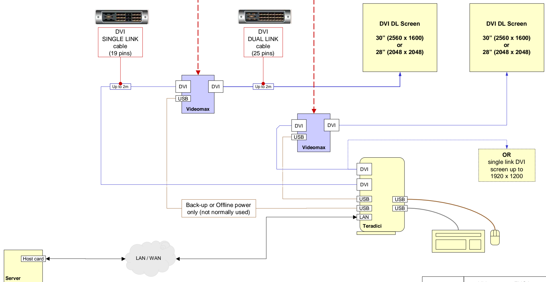
Figure 1 Videomax on EVGA portal Connection Diagram Copyright 2010 Thruput Limited DN 1001 Issue: 1.6 Date: 20 May 2010
