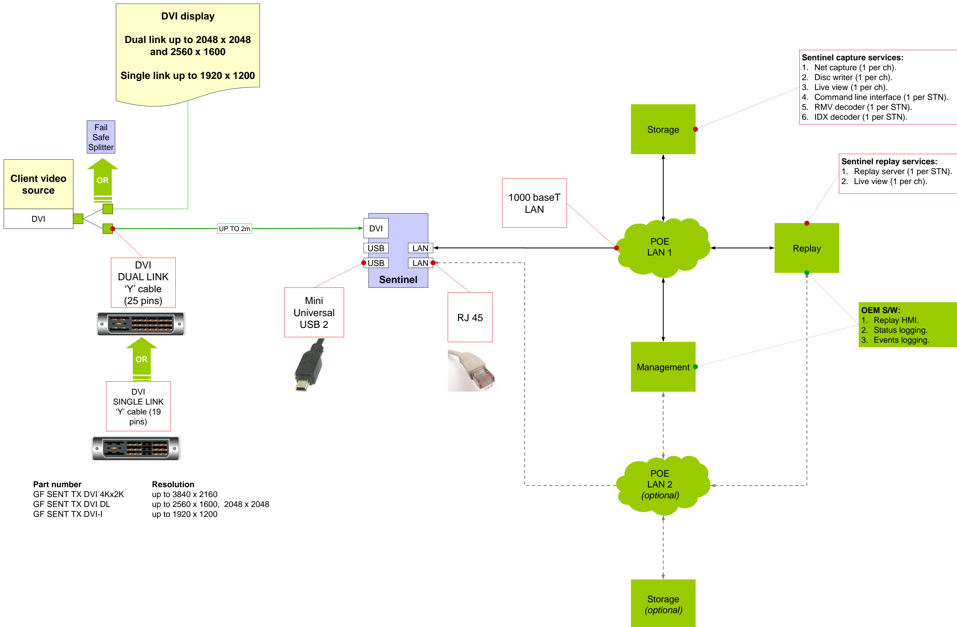
Figure 2 DVI DL or SL video
