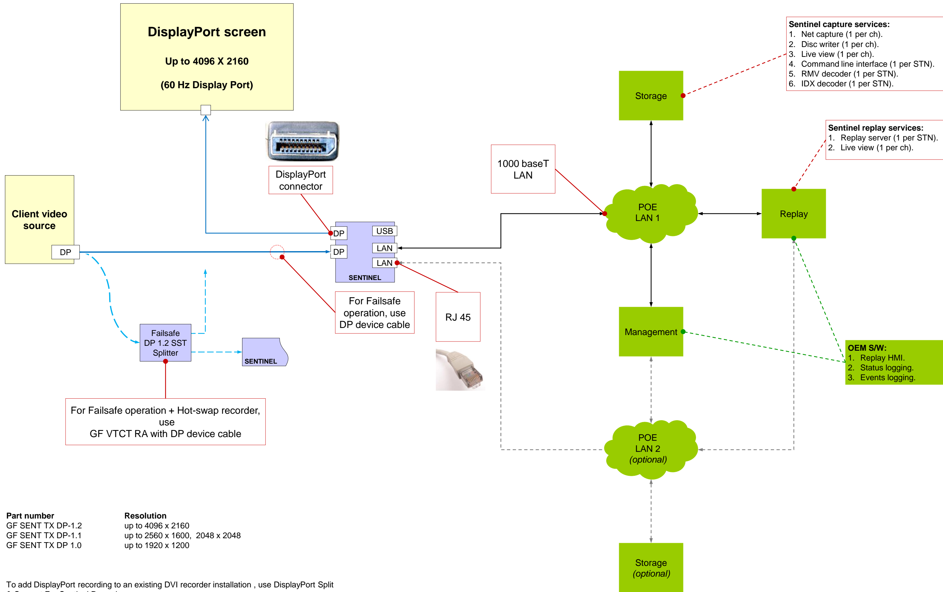
Figure 1 DisplayPort video
