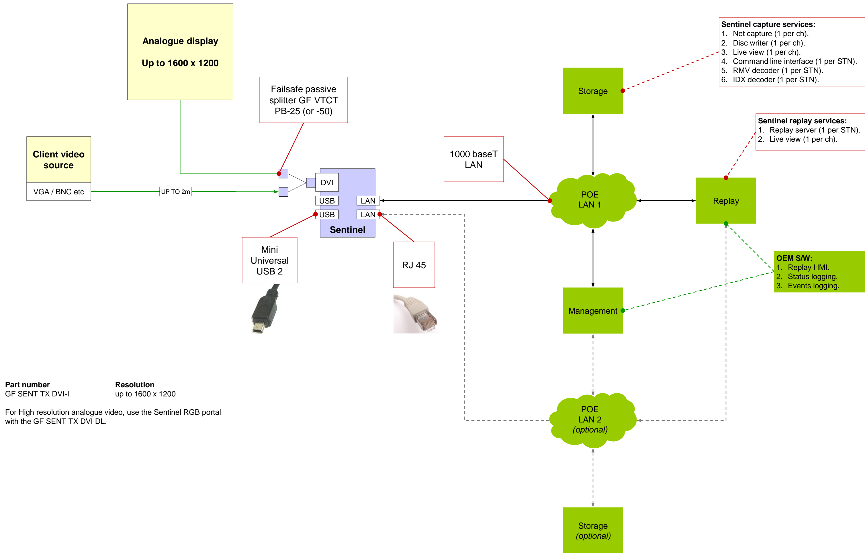
Figure 3 Analogue video
